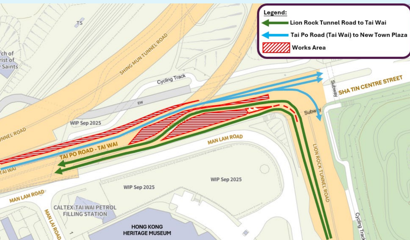
Temporary diversion: Left-turn from Lion Rock Tunnel Road towards Tai Po Road – Tai Wai
